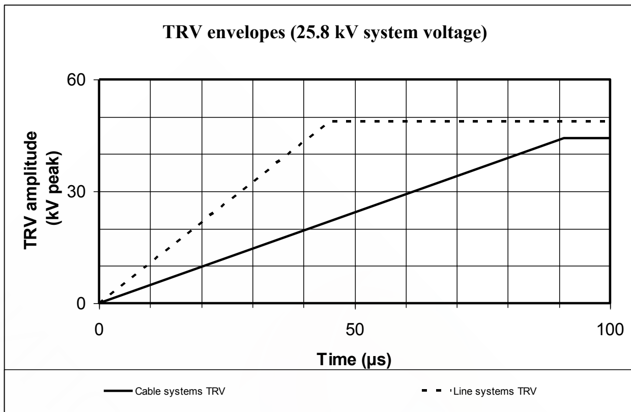
Figure F.1 Examples of TRV envelopes for two different system applications (overhead line and cable system) for circuit-breakers of the same system voltage rating (25.8 kV).
