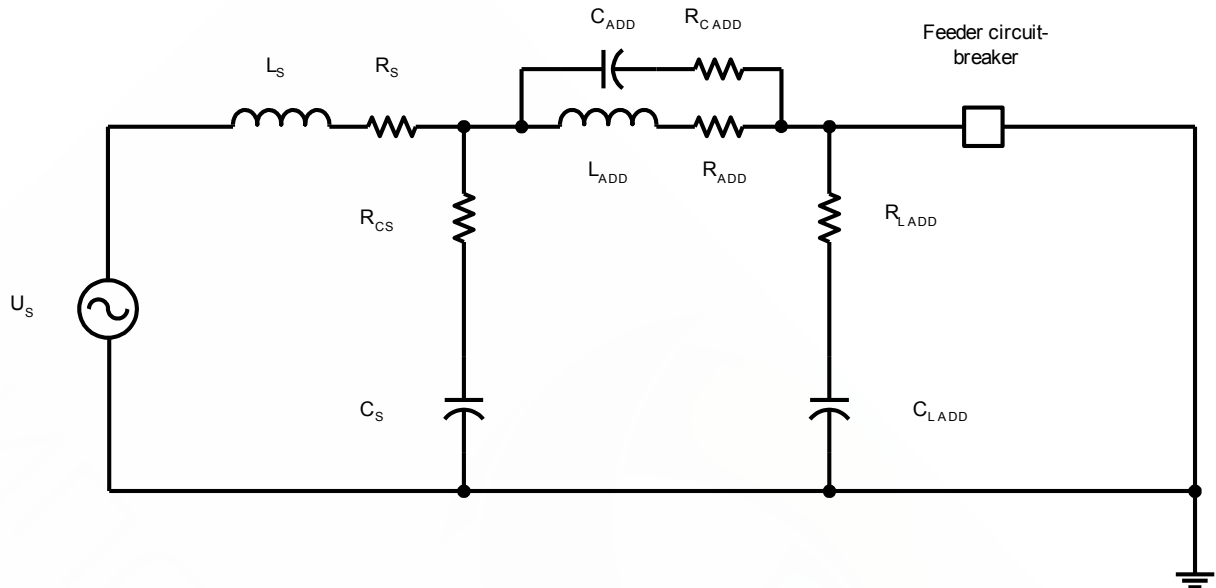
Figure F.3 Equivalent single-phase circuit used in the examples representing the first-pole-to-clear during a three-phase fault.
